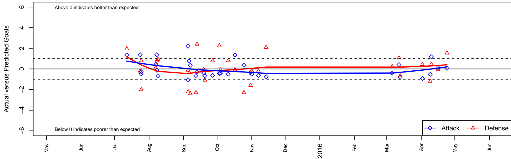
THUSC Titanium B01 Dots are actual minus expected GF (blue circles) and GA (red triangles). Blue line is smoothed change in attack strength. Red is smoothed change in defense strength.
